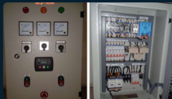
Panel Genset ATS AMF
